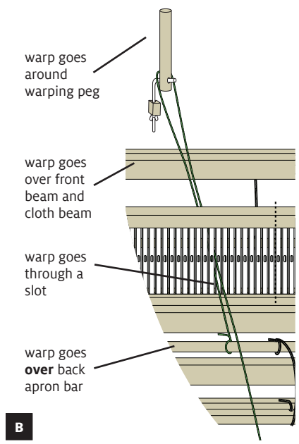
FIGURE 6: FIRST LOOP
