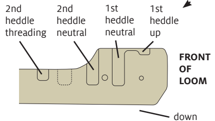
FIGURE 2: HEDDLE SLOTS
