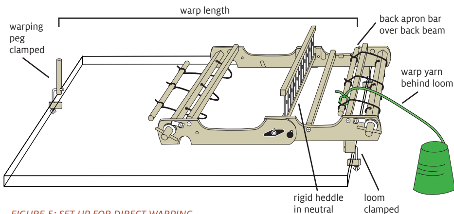
FIGURE 5: SET UP FOR DIRECT WARPING
