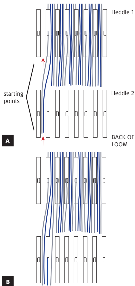
FIGURE 23: THREADING HEDDLE 2
