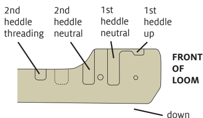
FIGURE 15: HEDDLE SLOTS
