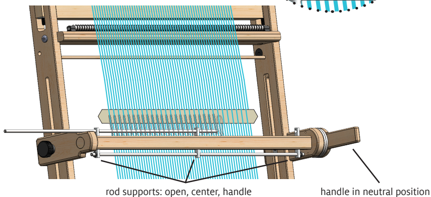
FIGURE 13: INSTALL HEDDLES
