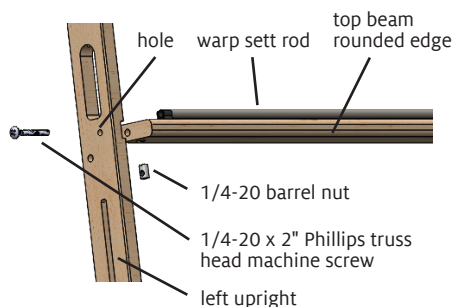
FIGURE 2: ATTACH THE TOP BEAM
