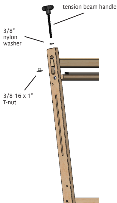
FIGURE 6: ADD HANDLES TO THE TENSION BEAM
