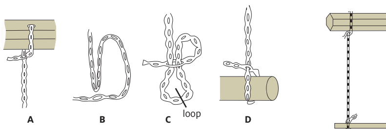
FIGURE 3: INSTALLING APRON CORDS
